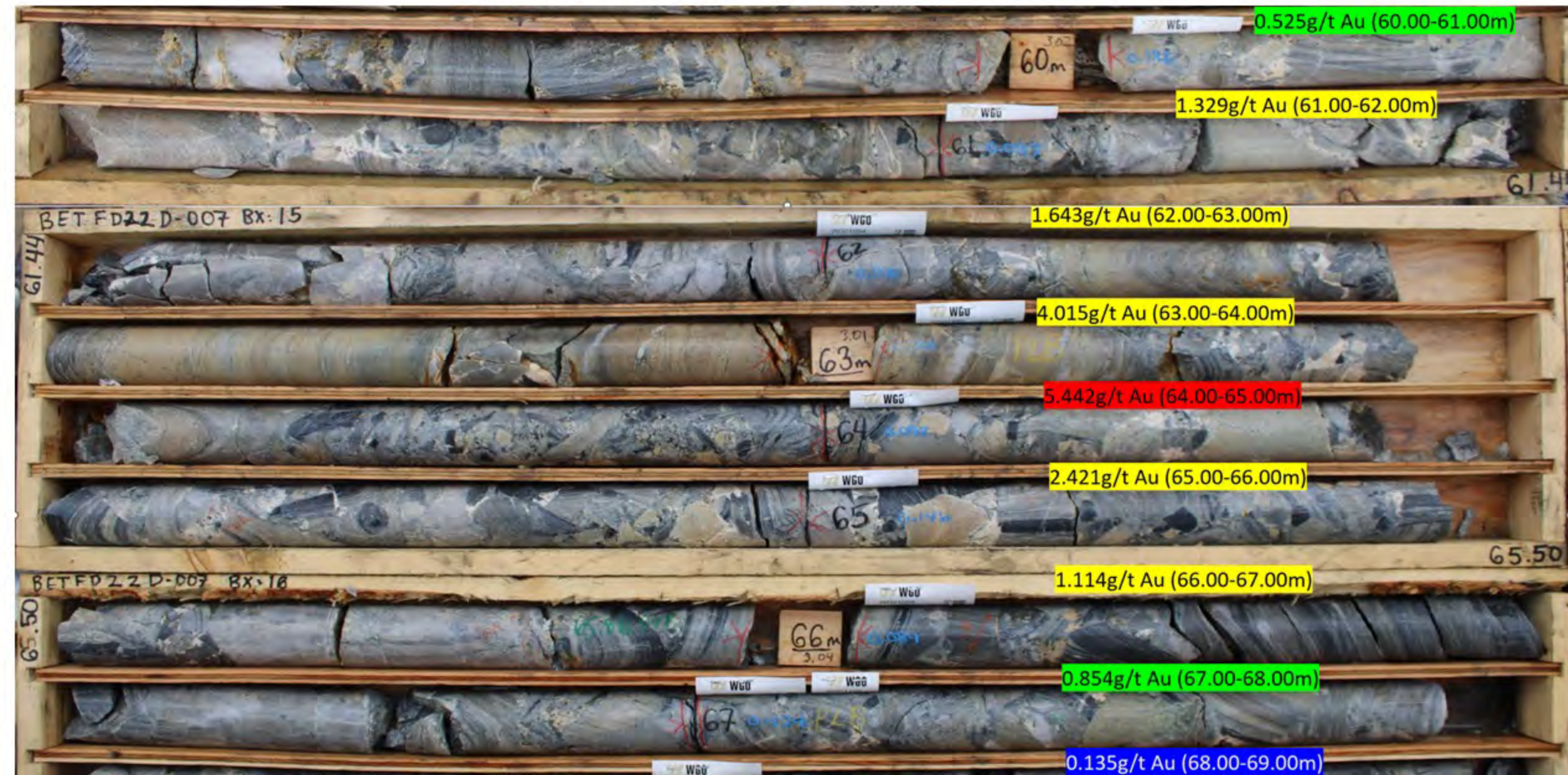
Figure 6: BETFD22D007 Core Photos – 60.0m to 69.0m
